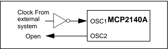
FIGURE 2-2: EXTERNAL CLOCK
